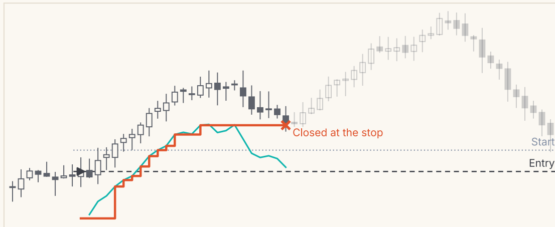
FIGURE 30 \text{ATR: stop loss} = \text{price} - 2 \times \text{ATR}(10)
